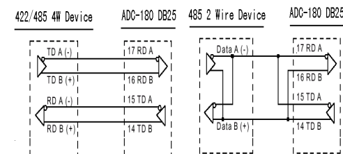
Figure 2: RS-422/485 Connection Diagrams
